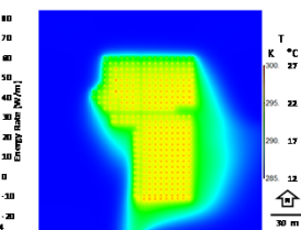
Figure 6. Three-dimensional heat distribution model of the wellfield in summer 2012 showing well-to-well interference and the influence of groundwater flow.
